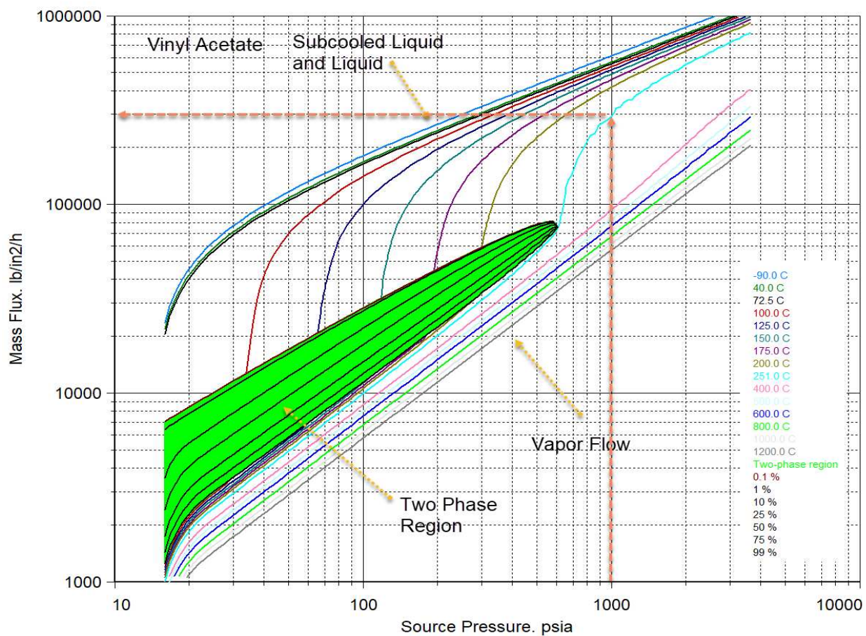
Figure 2: Vinyl acetate flow map generated by SuperChems Expert
