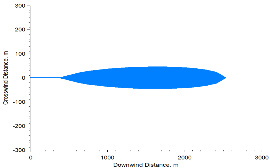
Figure 7: 500 ppm isopleth for elevated release
