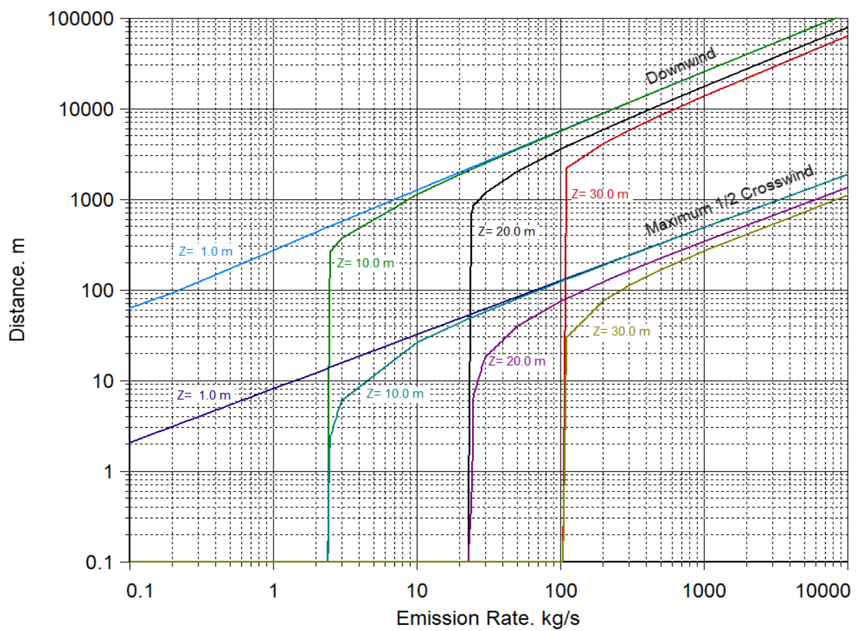
Figure 4: Dispersion chart at ERPG-2 equivalent dose for a 10 minute release of Vinyl Acetate. F stability. 2.6 m/s wind speed.
