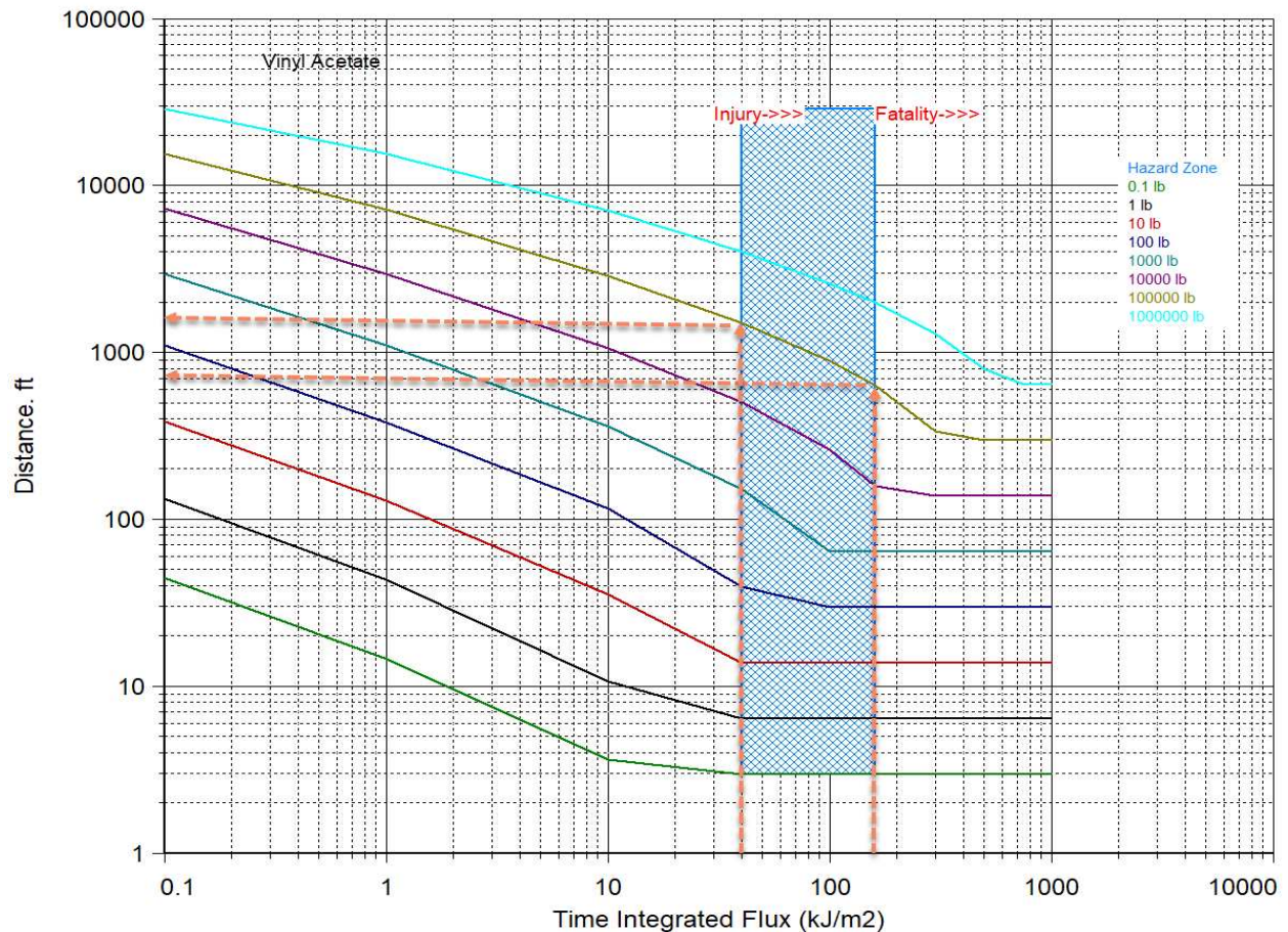
Figure 8: Thermal radiation hazards (fireball) for vinyl acetate
