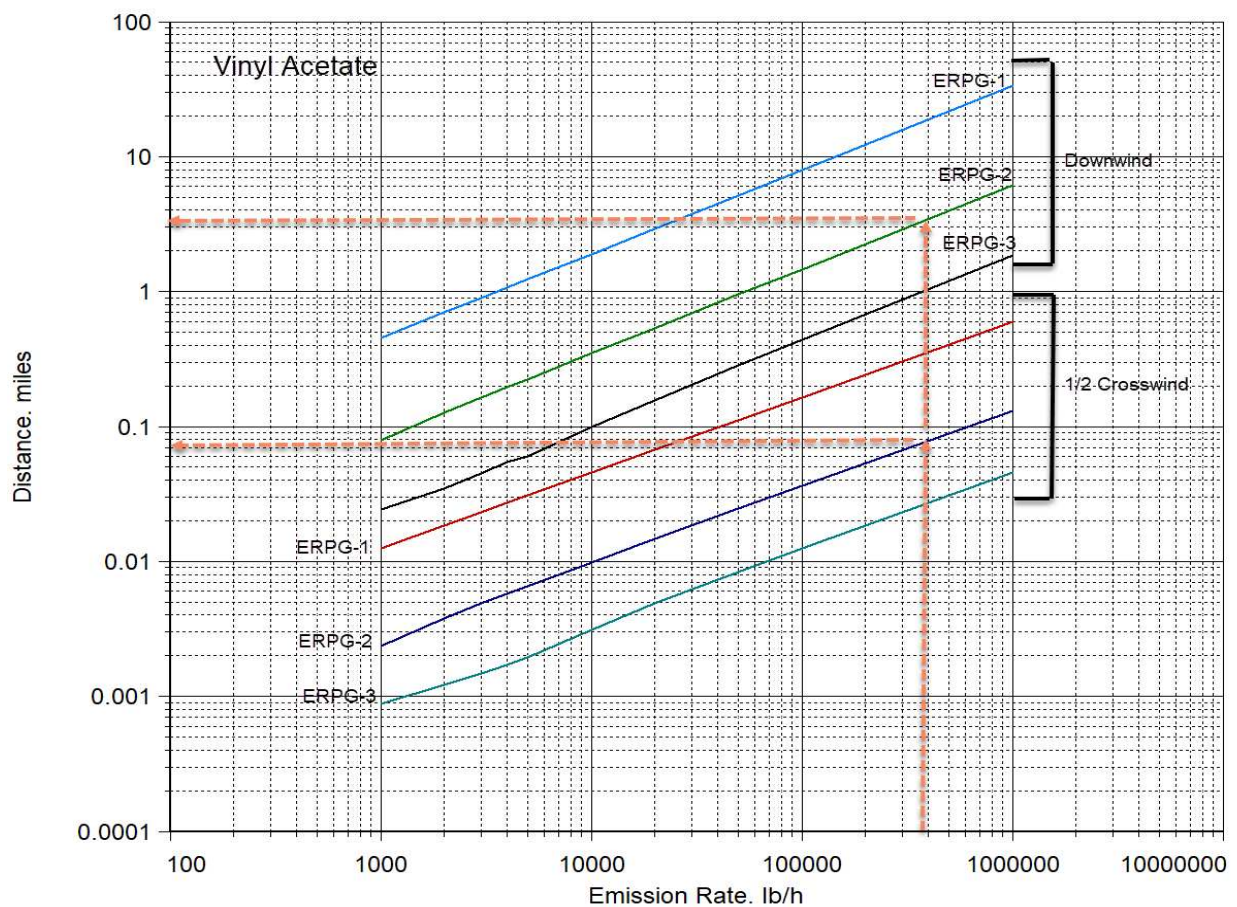
Figure 5: Dispersion chart at ERPG equivalent dose for a 10 minute release of Vinyl Acetate. F stability. 2.0 m/s wind speed.
