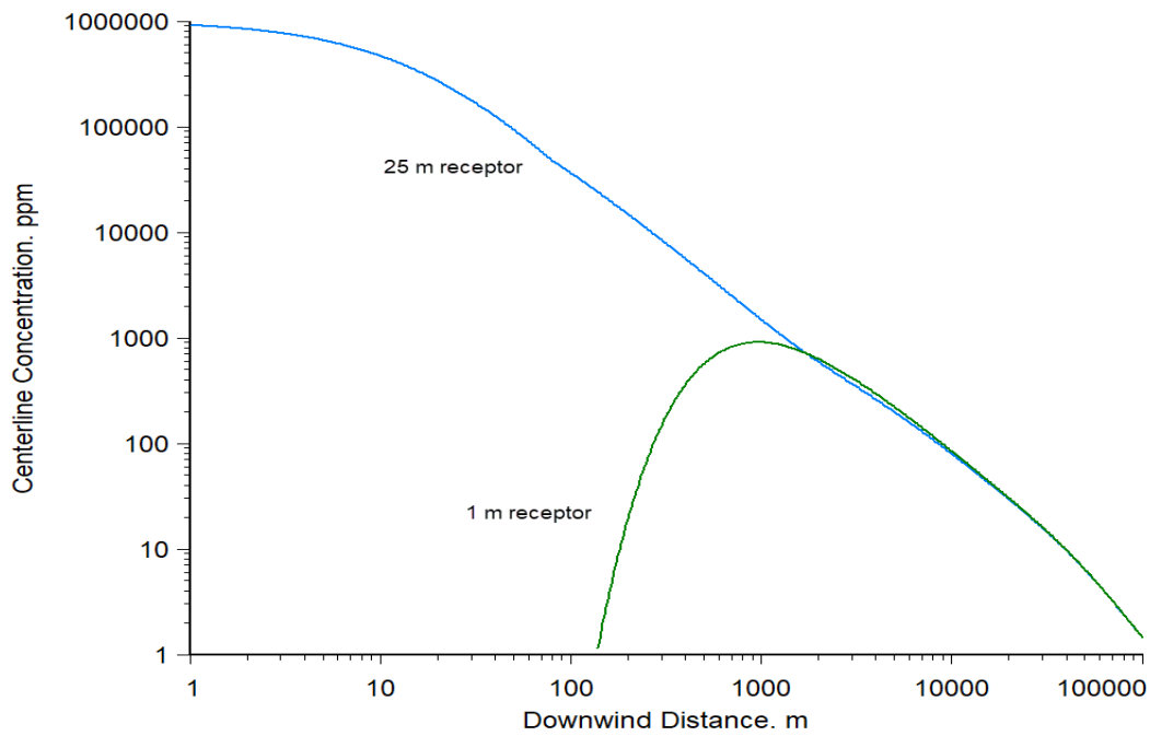
Figure 6: Typical Gaussian centerline concentration profile from an elevated release
