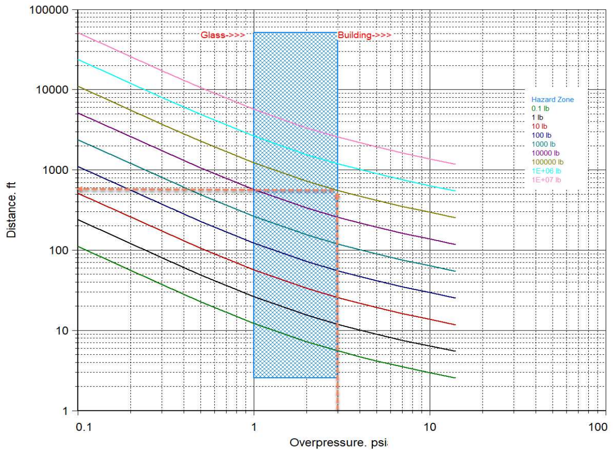
Figure 9: Overpressure hazards for vinyl acetate
