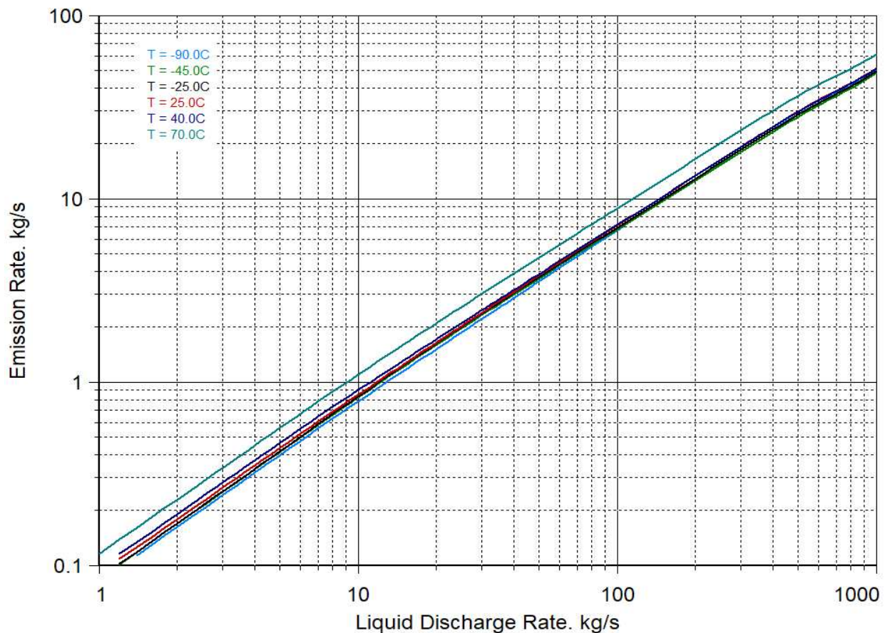
Figure 3: Pool vapor emission rate for a 10 minute liquid release of Vinyl Acetate. D stability. 4.5 m/s wind speed.
