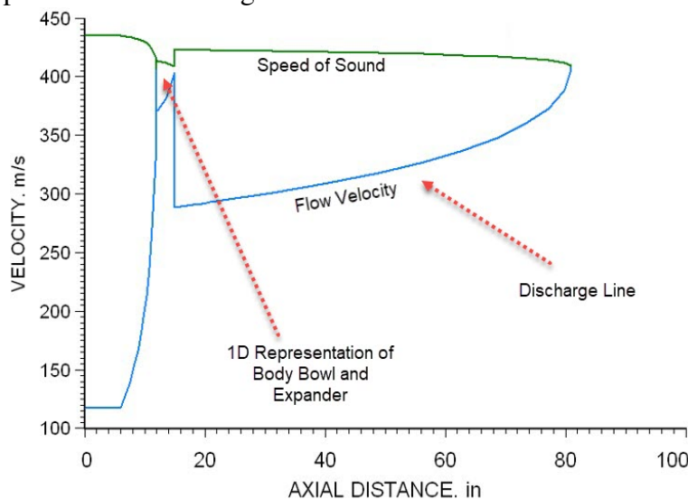
Figure 6: Body bowl choking for a gas system with an expander and a discharge line
