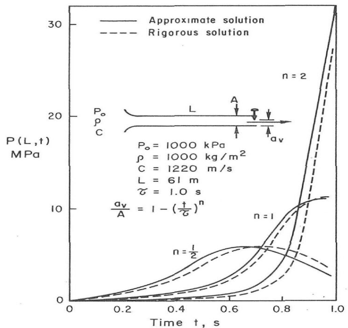
Figure 8: Moody's Waterhammer Solution
