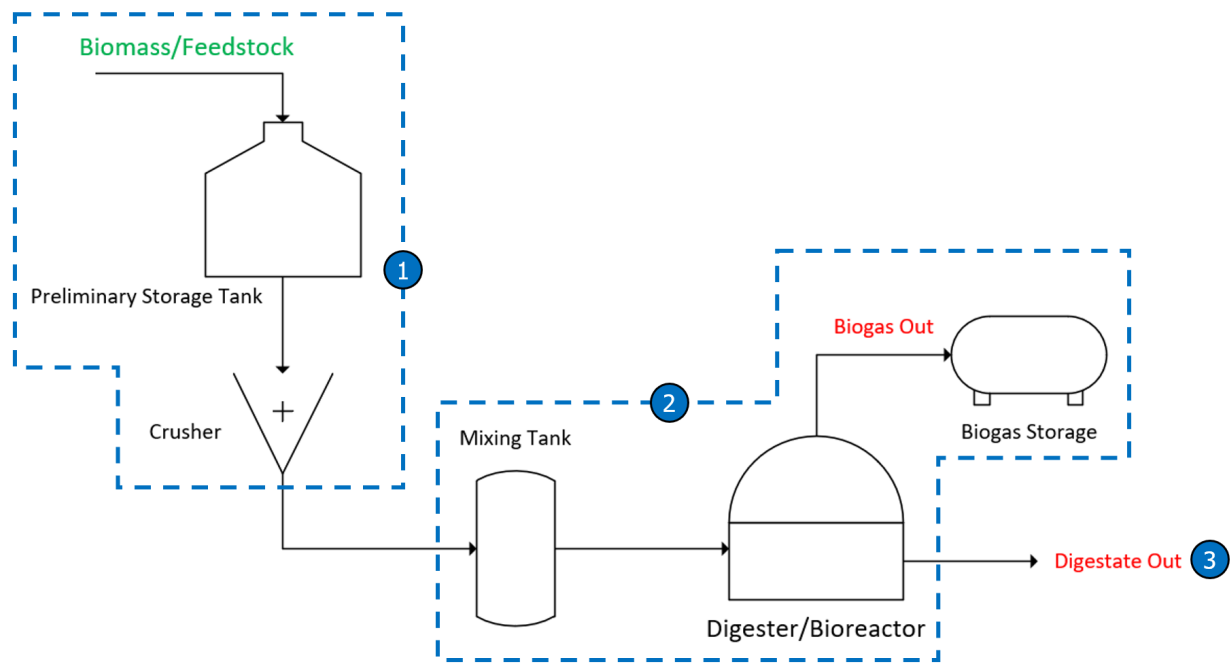
Figure 4: Simplified process flow diagram of biogas production
