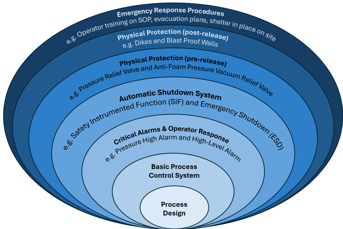
Figure 7: Example LOPA of a biogas facility
